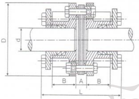
DJM(T)型胀紧套联结弹性膜片联轴器 DJM(T) Type Bioated set binding elastic diaphragm Shaft coupling
