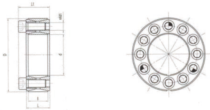
基本尺寸和参数 Basic dimensions and parameters of the locking assemblies, type Z2
