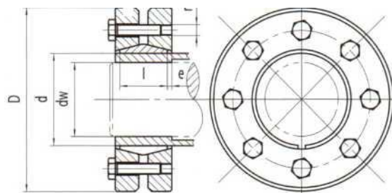
基本尺寸和参数 Basic dimensions and parameters of the locking assemblies,type Z7C
