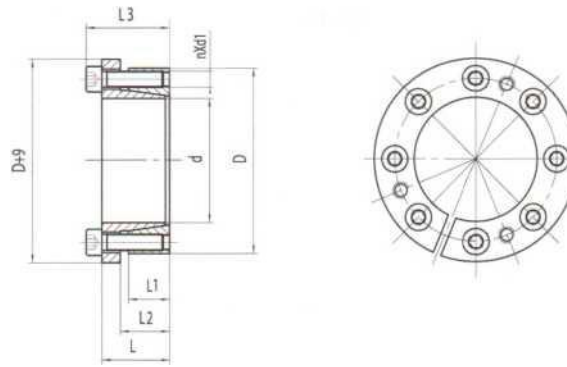
基本尺寸和参数 Basic dimensions and parameters of the locking assemblies,type Z9
