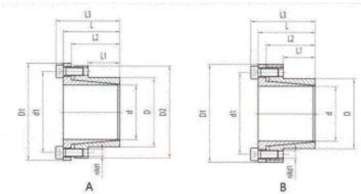
基本尺寸和参数 Basic dimensions and parameters of the locking assemblies,type Z11A/B
