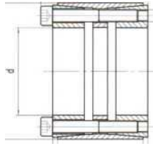
基本尺寸和参数 Basic dimensions and parameters of the locking assemblies, type Z12A
