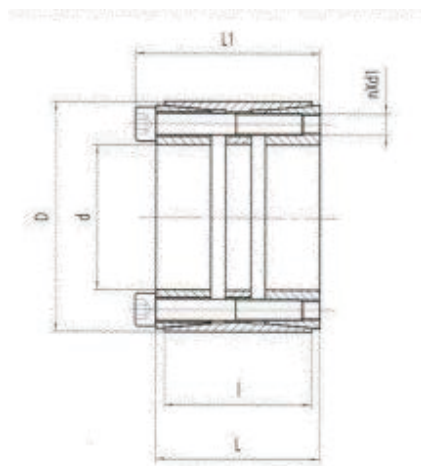
基本尺寸和参数 Basic dimensions and parameters of the locking assemblies,type Z12B
