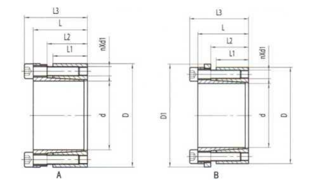
基本尺寸和参数 Basic dimensions and parameters of the locking assemblies,type Z13A/B
