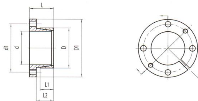
基本尺寸和参数 Basic dimensions and parameters of the locking assemblies,type Z14A
