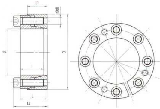
基本尺寸和参数 Basic dimensions and parameters of the locking assemblies, type Z15
