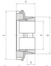
基本尺寸和参数 Basic dimensions and parameters of the locking assemblies, type Z19A
