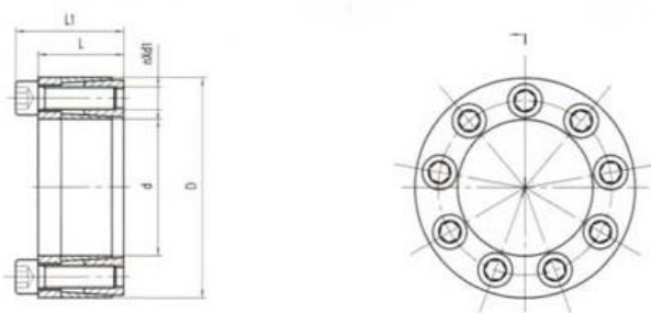
基本尺寸和参数 Basic dimensions and parameters of the locking assemblies,type Z22
